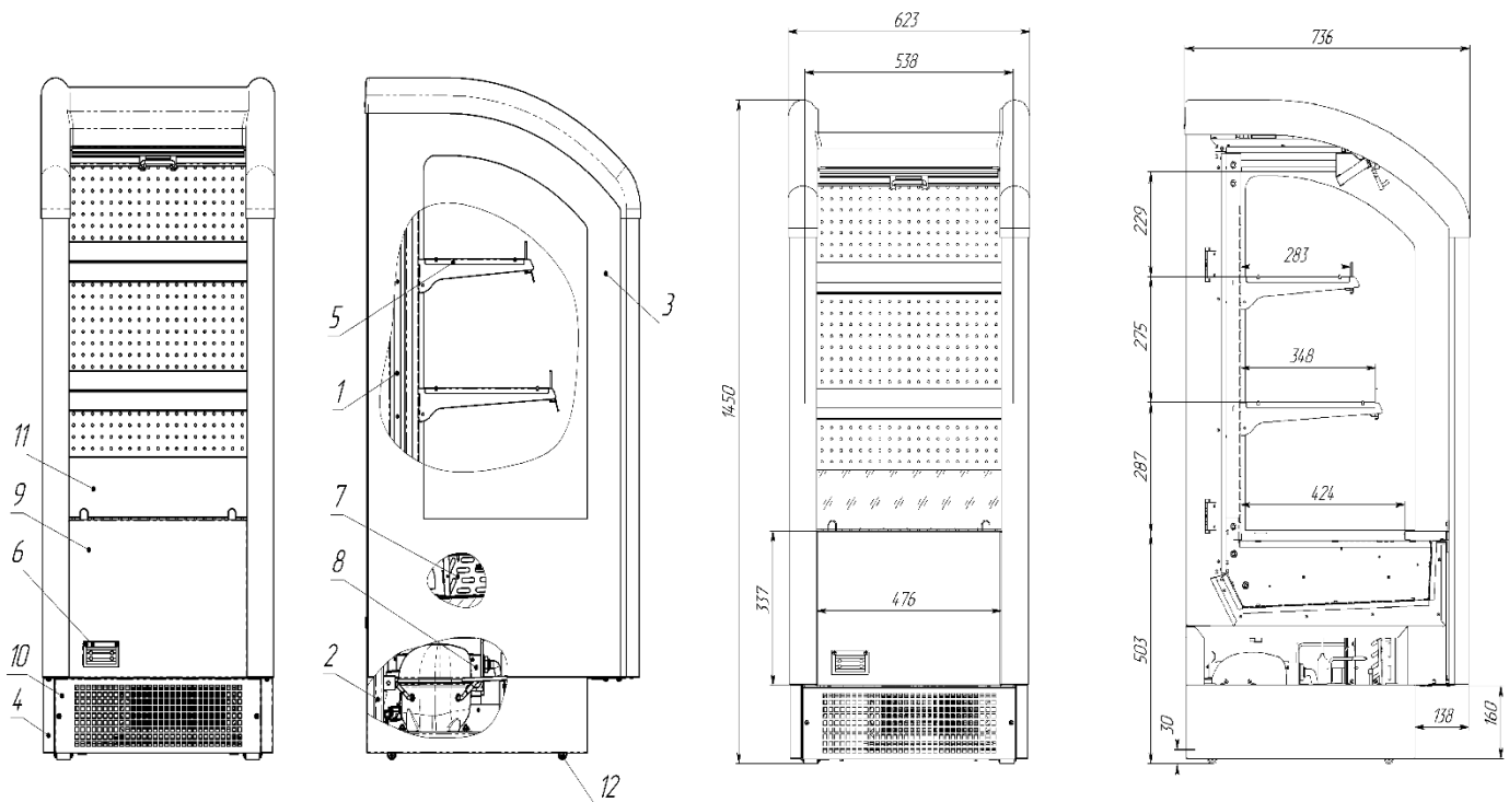
Figure 2 – Arrangement of major units and components
