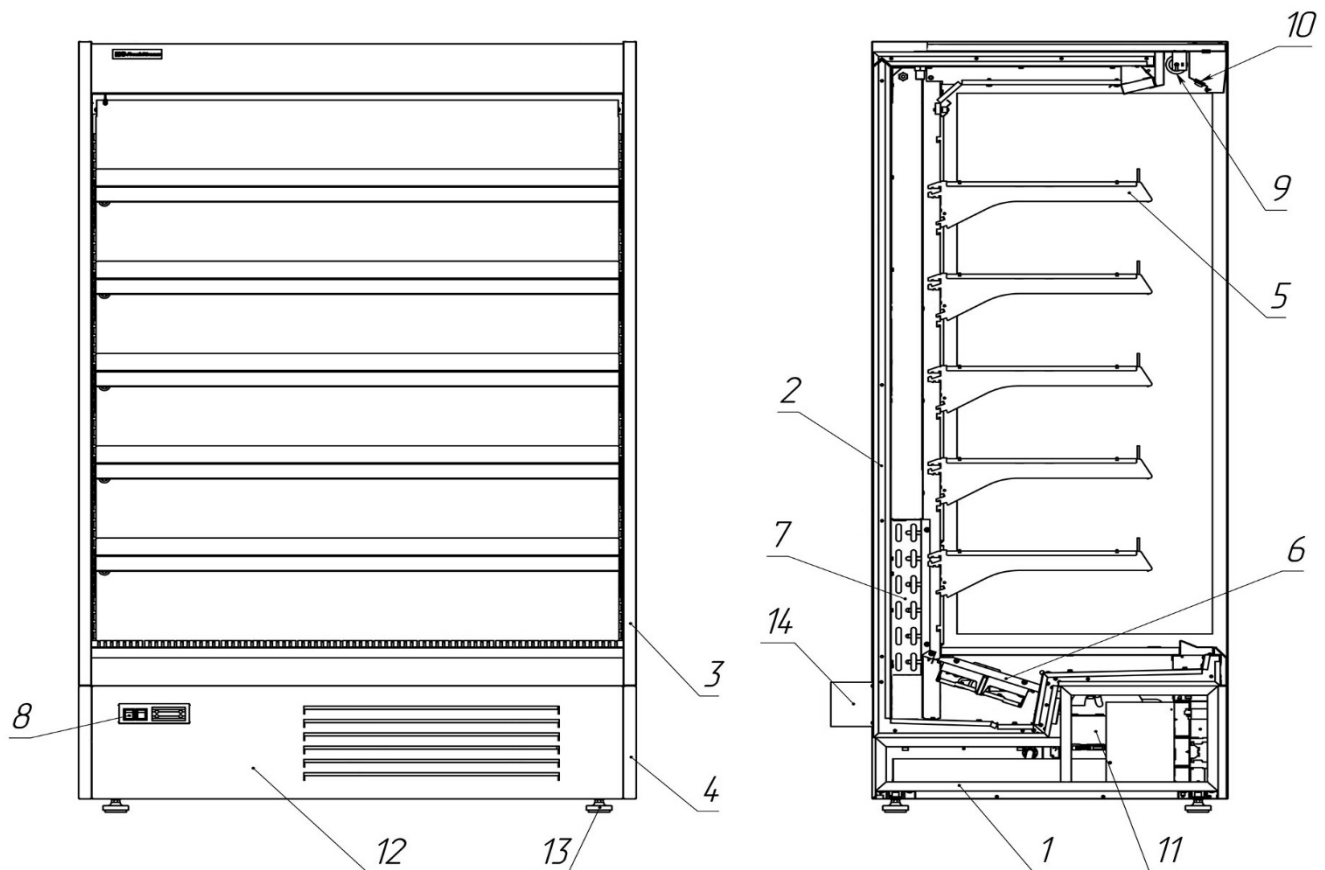
Figure 2 – Arrangement of major units and components
